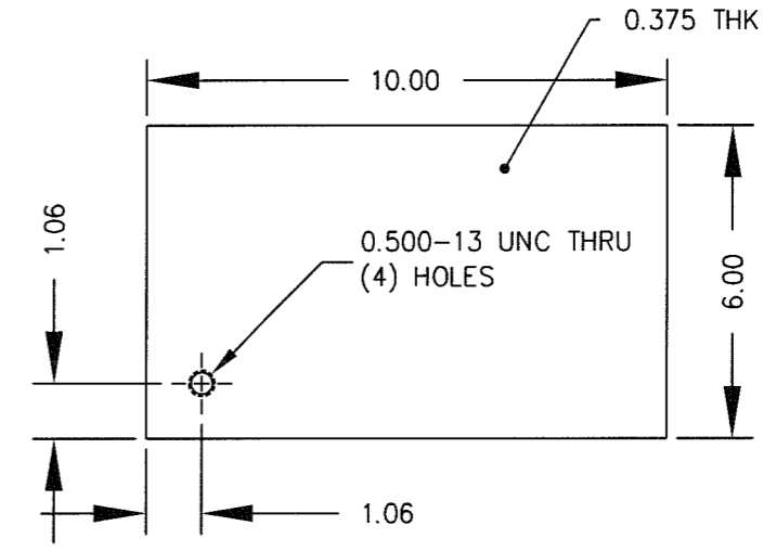
ITEM #2 CORNER PLATE SCALE 1:2
